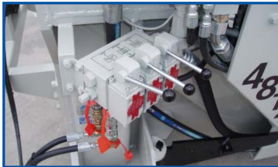
Low pressure valves for hydraulic make-up tool, push plate brake, and staging functions.
